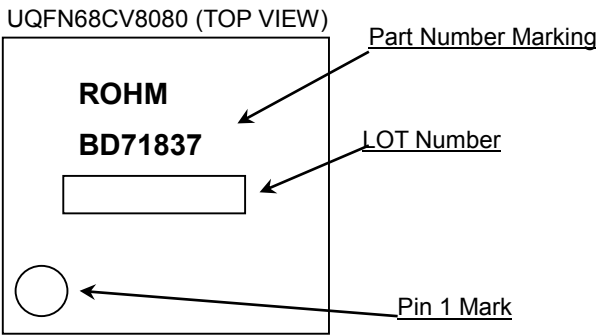
Figure 9-1. Marking Diagram
