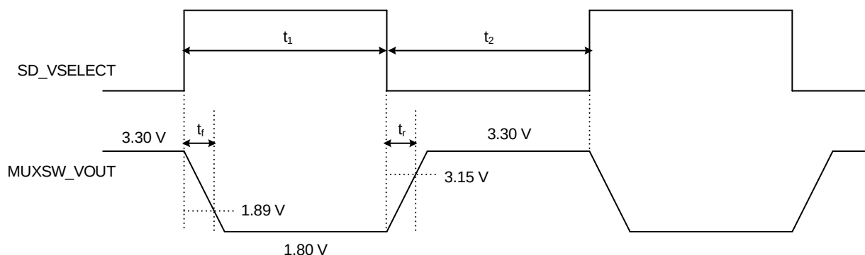
Figure 5-19. MUXSW Sequence
