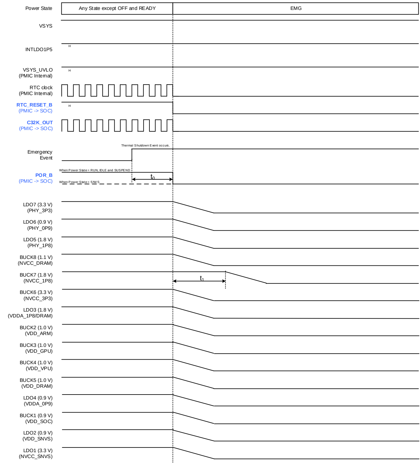
Figure 3-29. Emergency Shutdown
