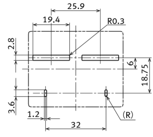
Recommended PC board pattern (BOTTOM VIEW)
