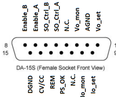
Figure 1a. Signal Connector
