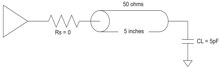
Figure 1. Test Circuit
