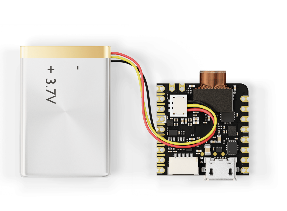
Example of a typical solution for remote machine vision including an Arduino® Nicla Vision and battery. Notice the orientation of the battery's cable in the board's connector.
