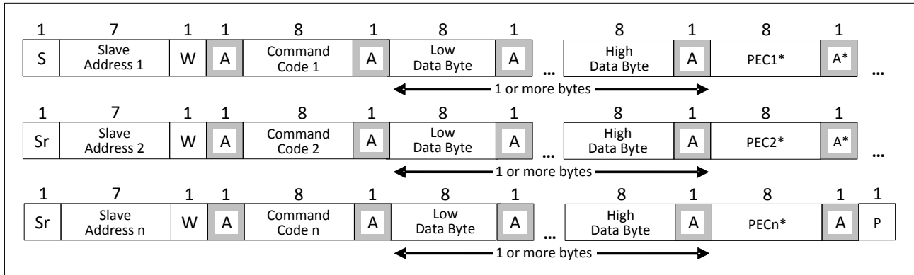
Figure 64: Group Command
