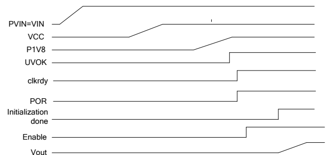
Figure 11: IR38063 Initialization sequence
