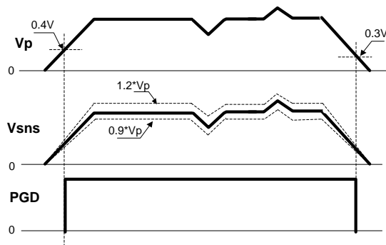
Figure 30: Vp Tracking ( \text{Track\_En} = 0\text{V} )
