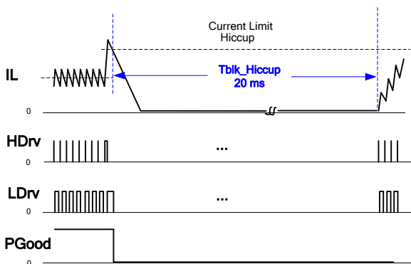
Figure 21: Timing Diagram for Current Limit Hiccup
