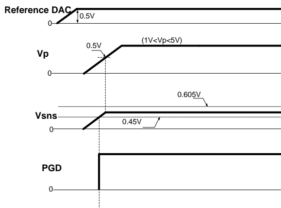
Figure 31: Vp Sequencing ( \text{Track\_En} = \text{Float} )
