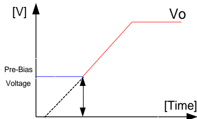
Figure 16: Pre-Bias startup
