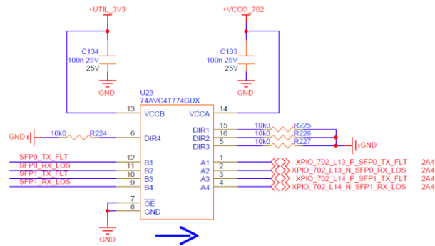
Figure 29 – SFP28 Voltage Translation
