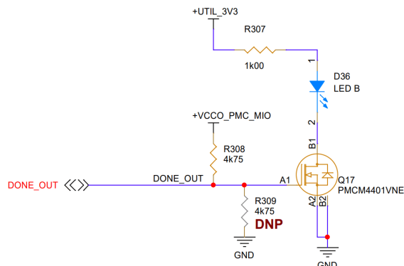
Figure 8 – DONE_OUT LED Schematic
