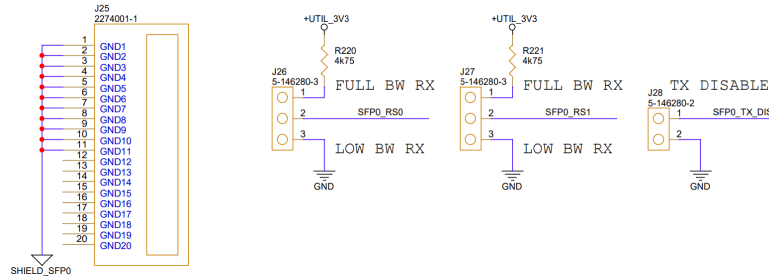
Figure 28 – SFP28 Cage and Jumpers Schematic
