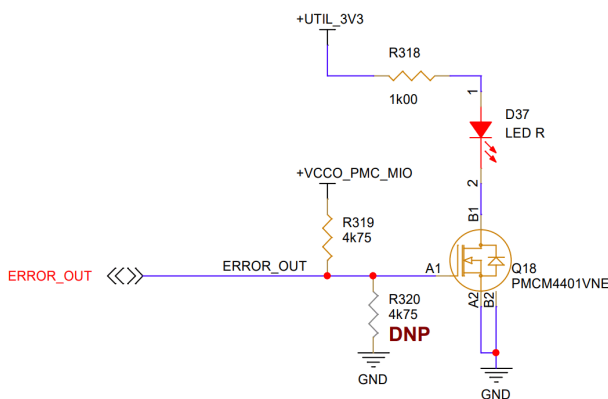
Figure 9 – ERROR_OUT LED Schematic
