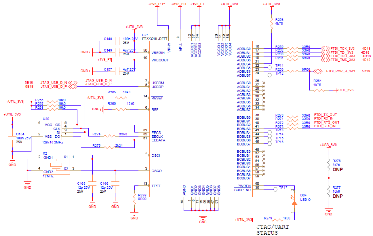
Figure 18 – USB JTAG-UART Schematic
