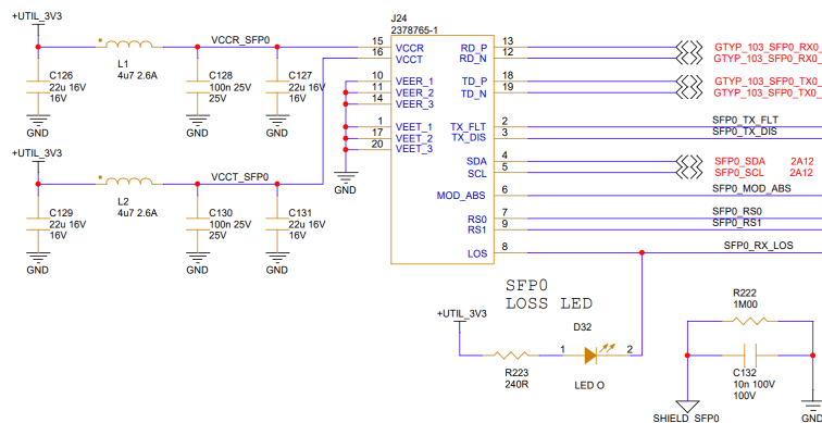
Figure 27 – SFP28 Interface Connector Schematic
