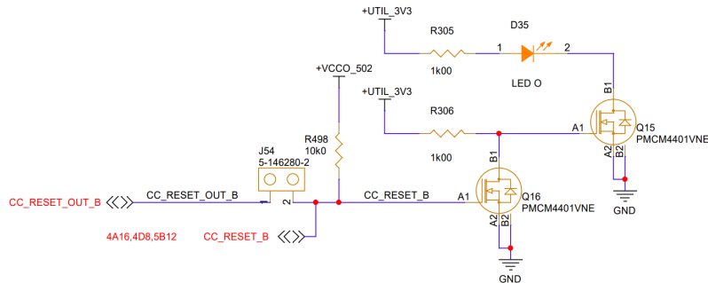
Figure 7 – CC_RESET_OUT_B LED Schematic
