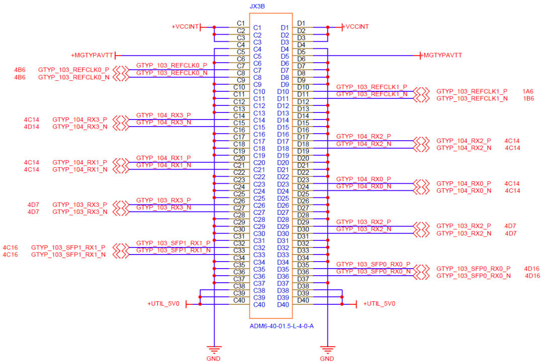
Figure 26 – JX3 Row C/D Carrier Card Pinout
