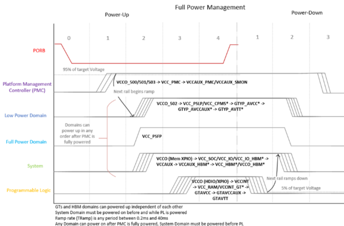
Figure 55 – Versal Power-On Sequence
