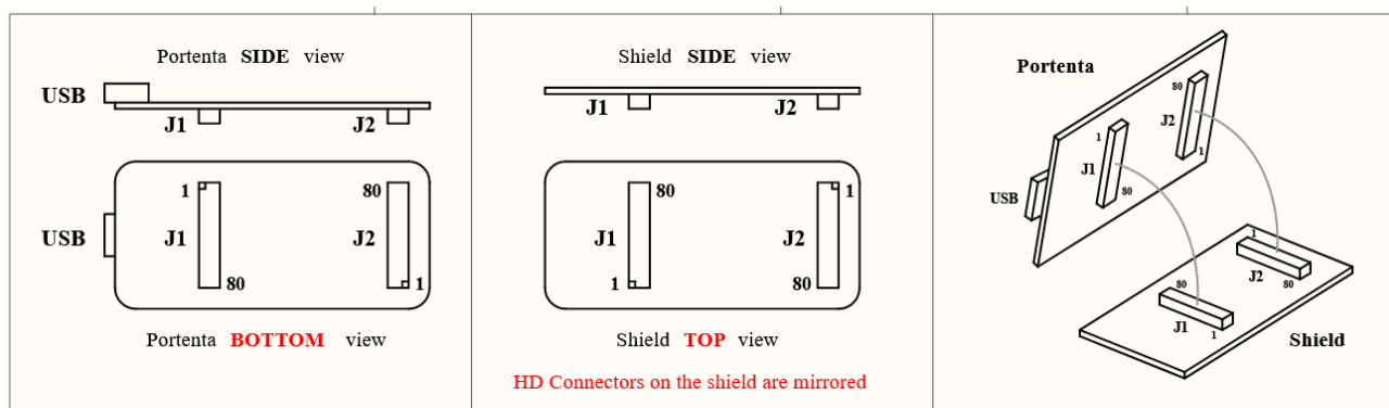
Mounting details
