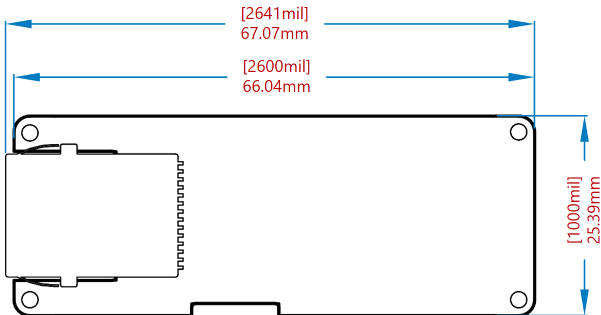
Board dimensions
