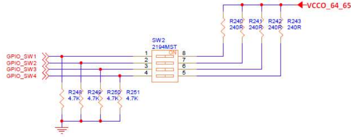
Figure 27 – User Dip Switch
