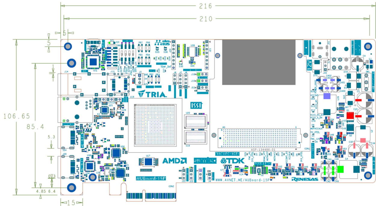
Figure 36 – Mechanical Dimensions
