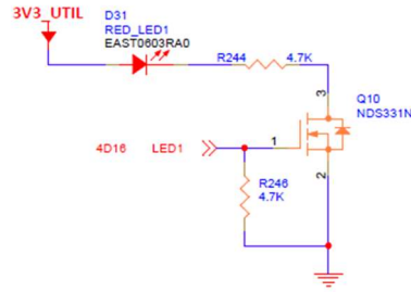
Figure 25 – RED User LED
