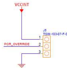
Figure 5 – POR_OVERRIDE Header
