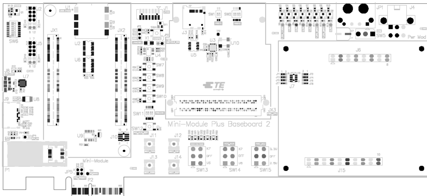
Figure 19 - Board Assembly Drawing
