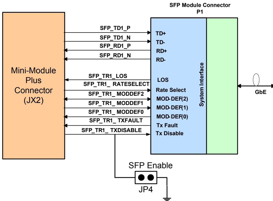
Figure 7 - SFP Module Interface
