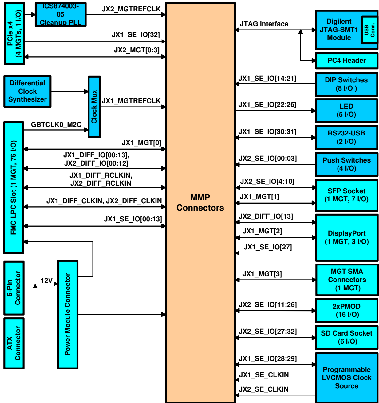
Figure 2 - Avnet Mini-Module Plus Baseboard 2 Block Diagram
