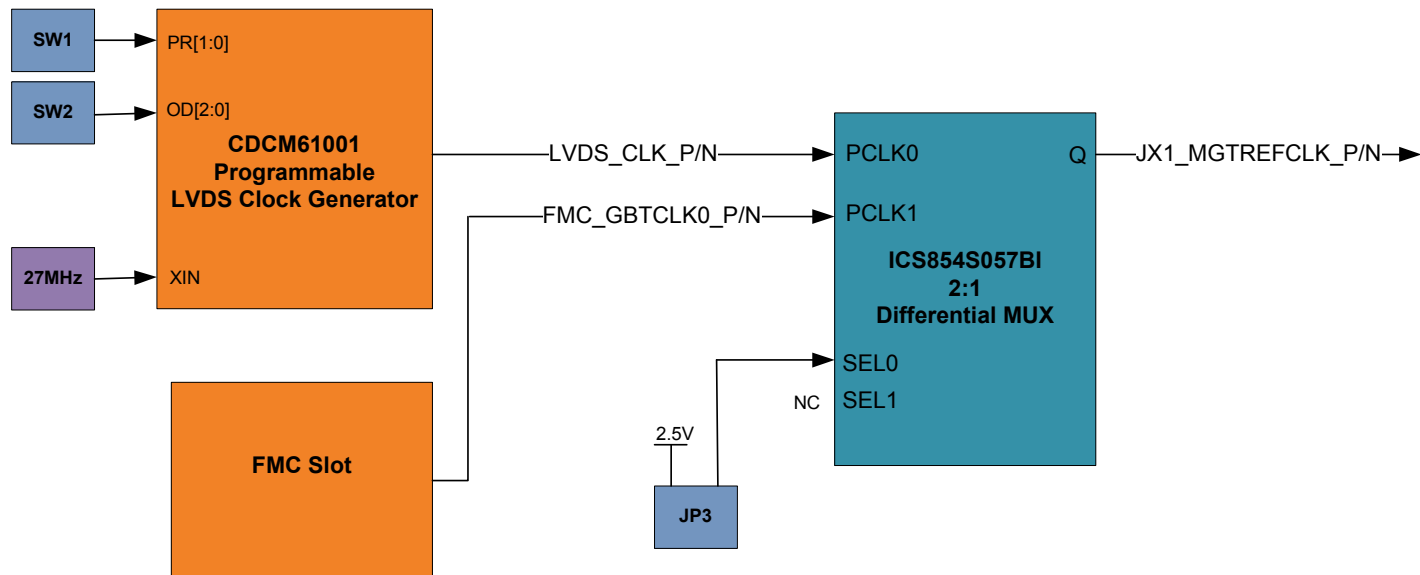
Figure 3 – GTX Reference Clock Sources
