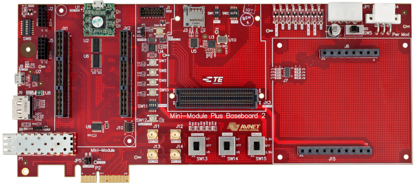
Figure 1 – Mini-Module Plus Baseboard 2 Picture
