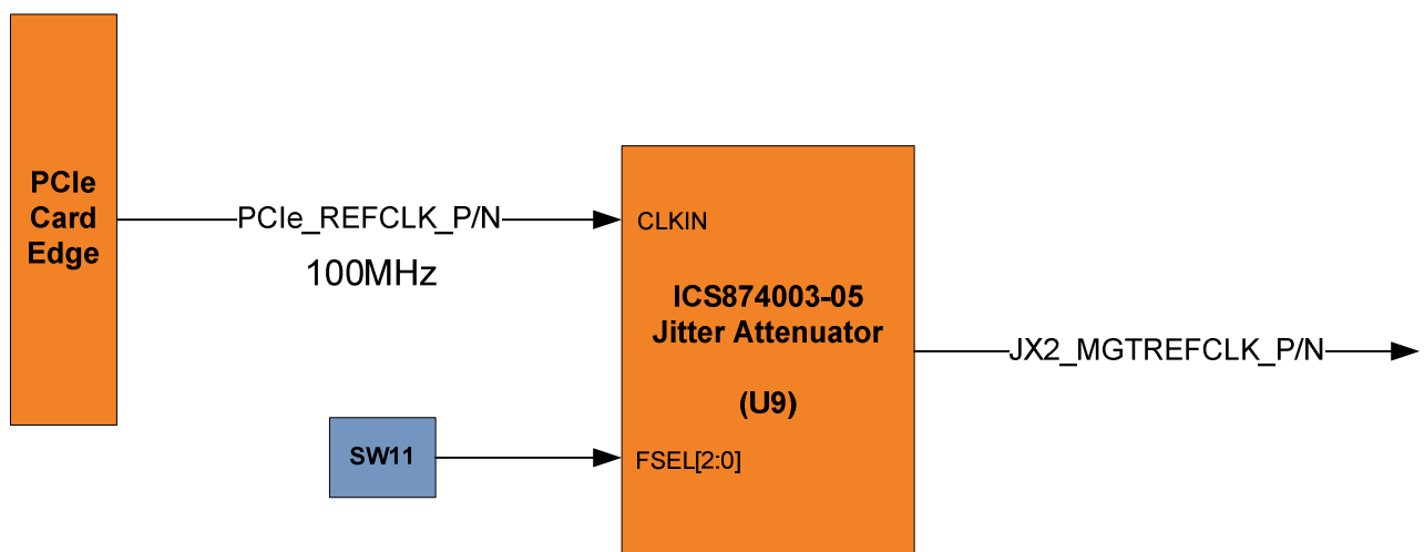
Figure 4- PCI Express Reference Clock
