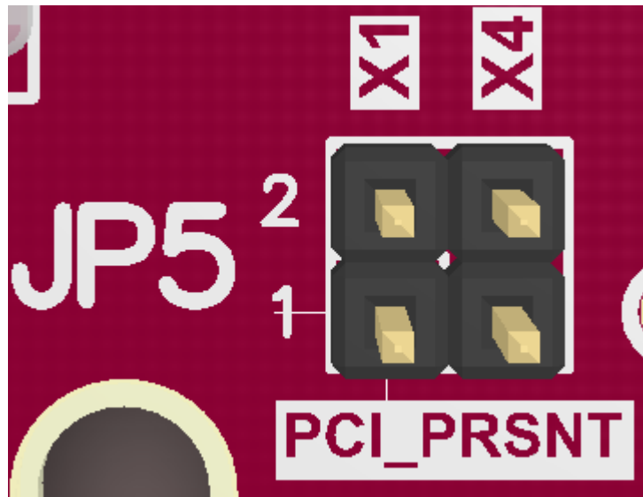
Figure 6 – PCI_PRSNT Configuration Jumper
