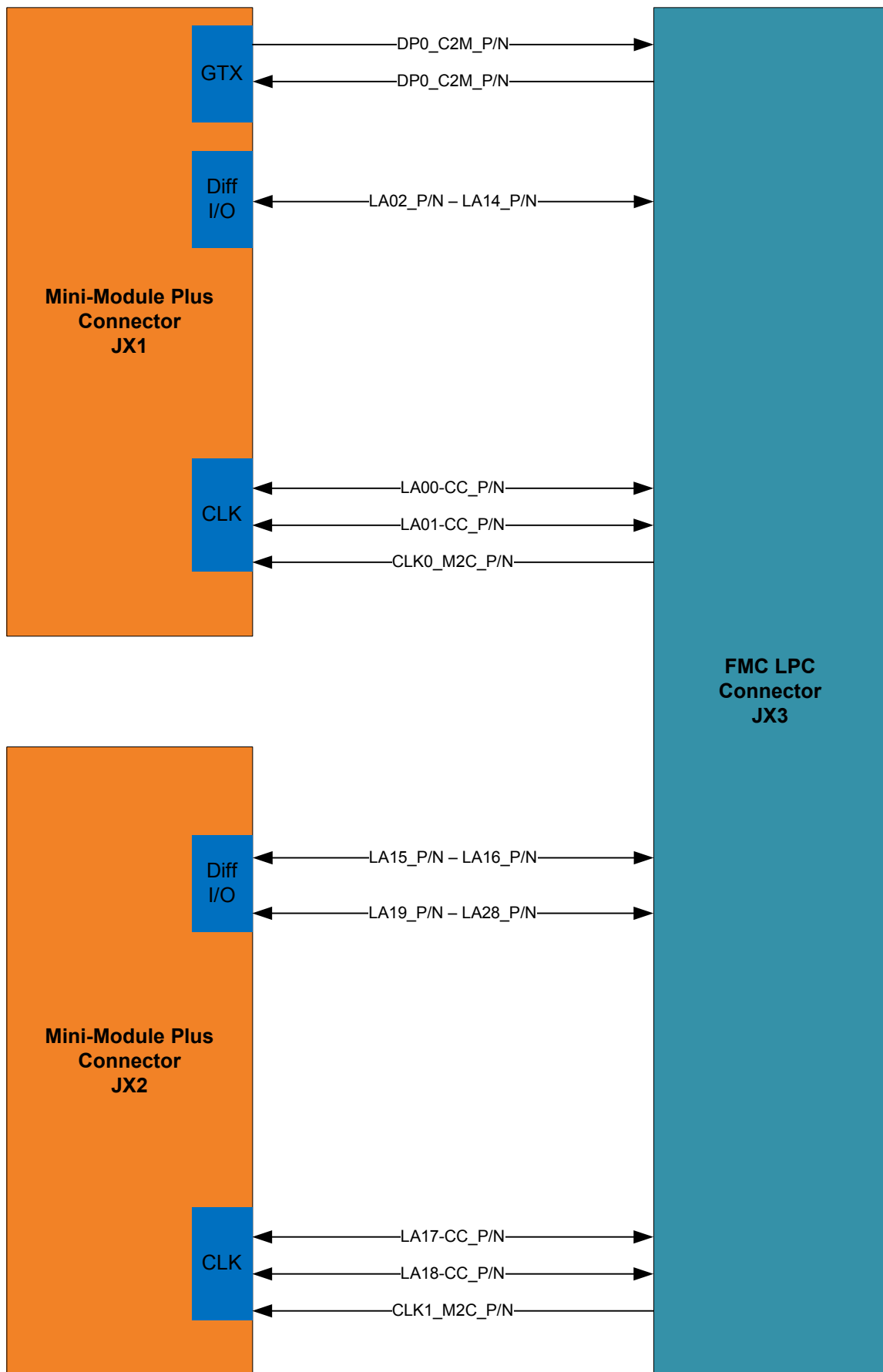
Figure 10 - FMC LPC Connector JX3 Block Diagram
