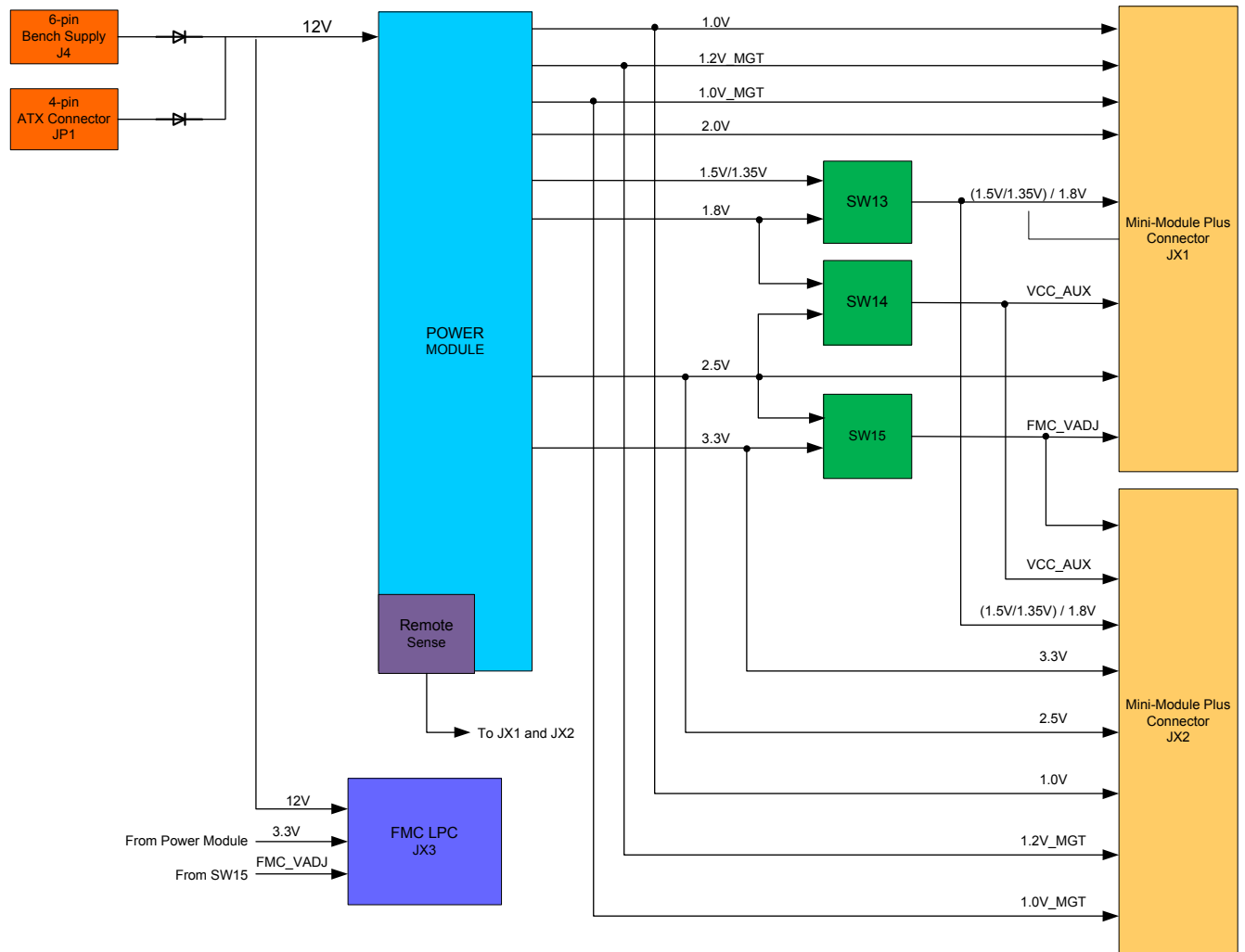
Figure 13 - Board Power
