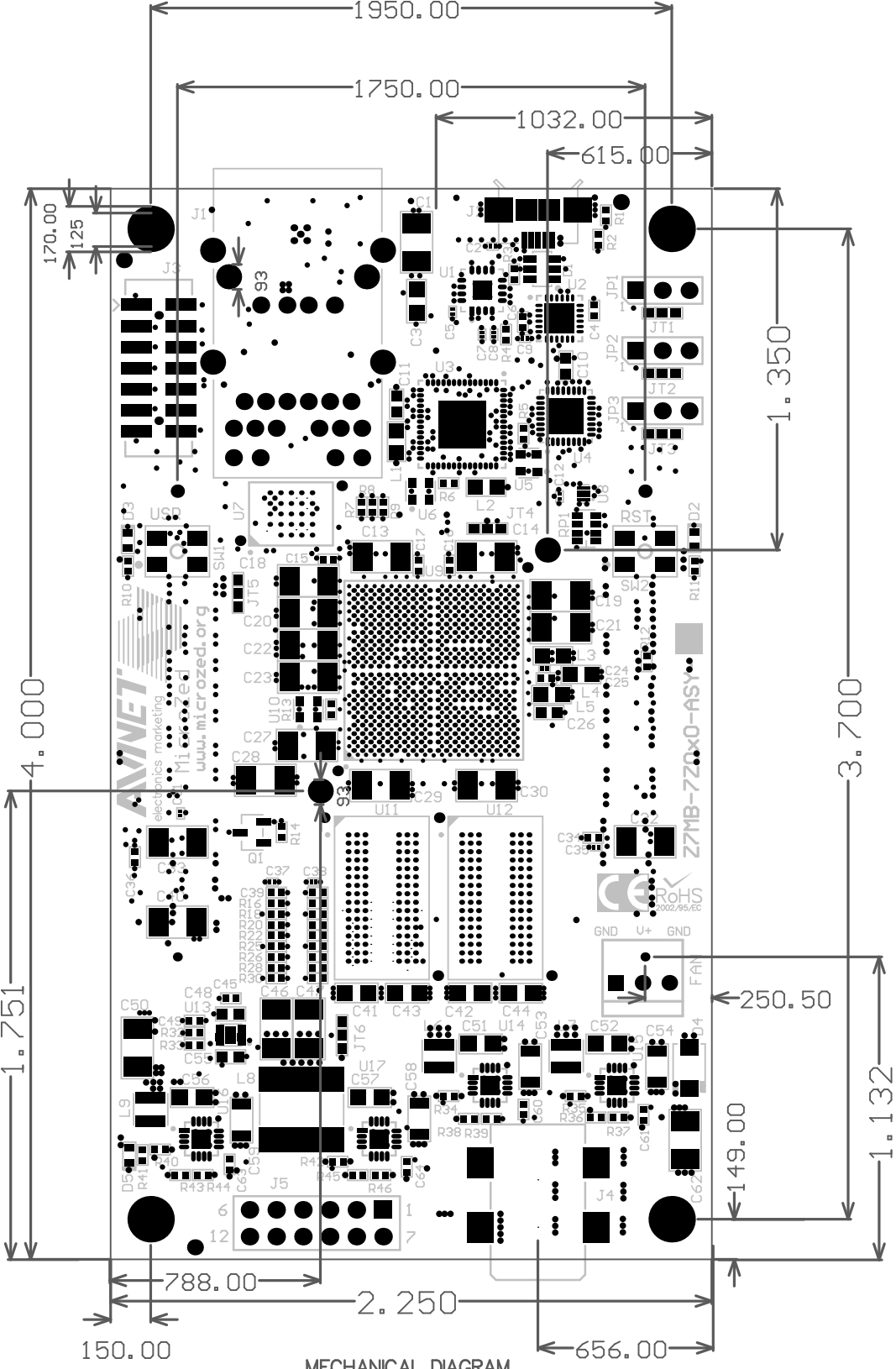
MECHANICAL DIAGRAM
