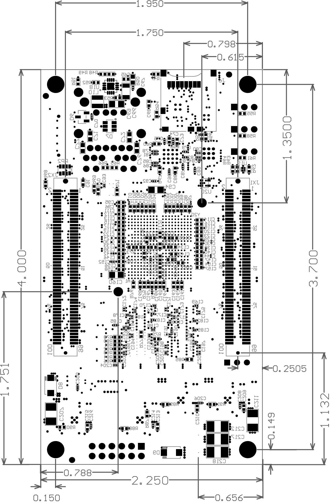
MECHANICAL DIAGRAM - ALL UNITS IN INCHES
