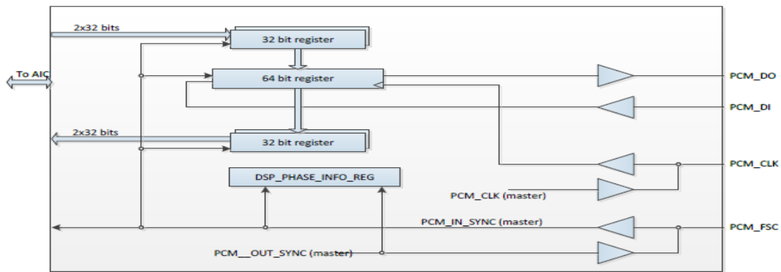
Figure 44 PCM controller
