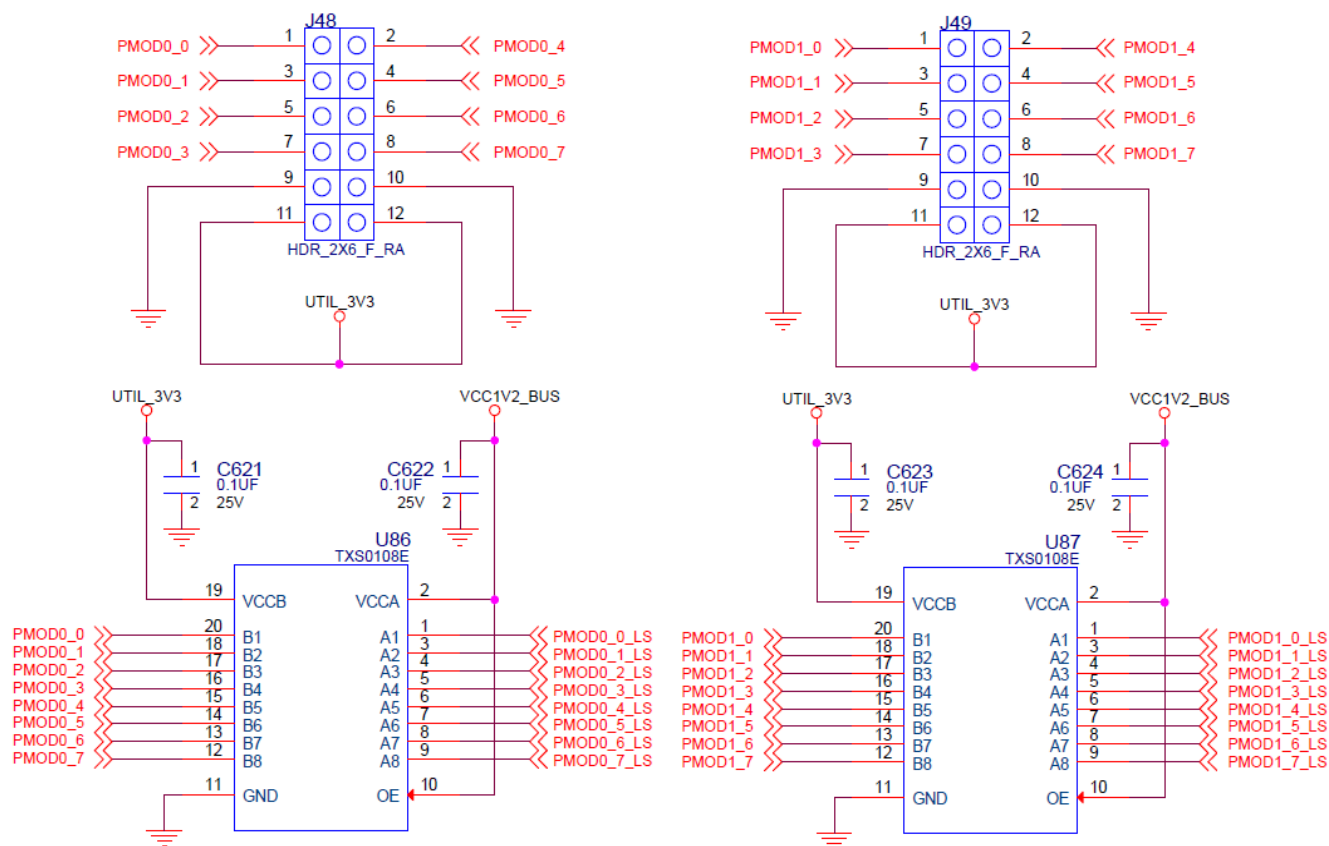
Figure 3-24: PMOD Connectors
