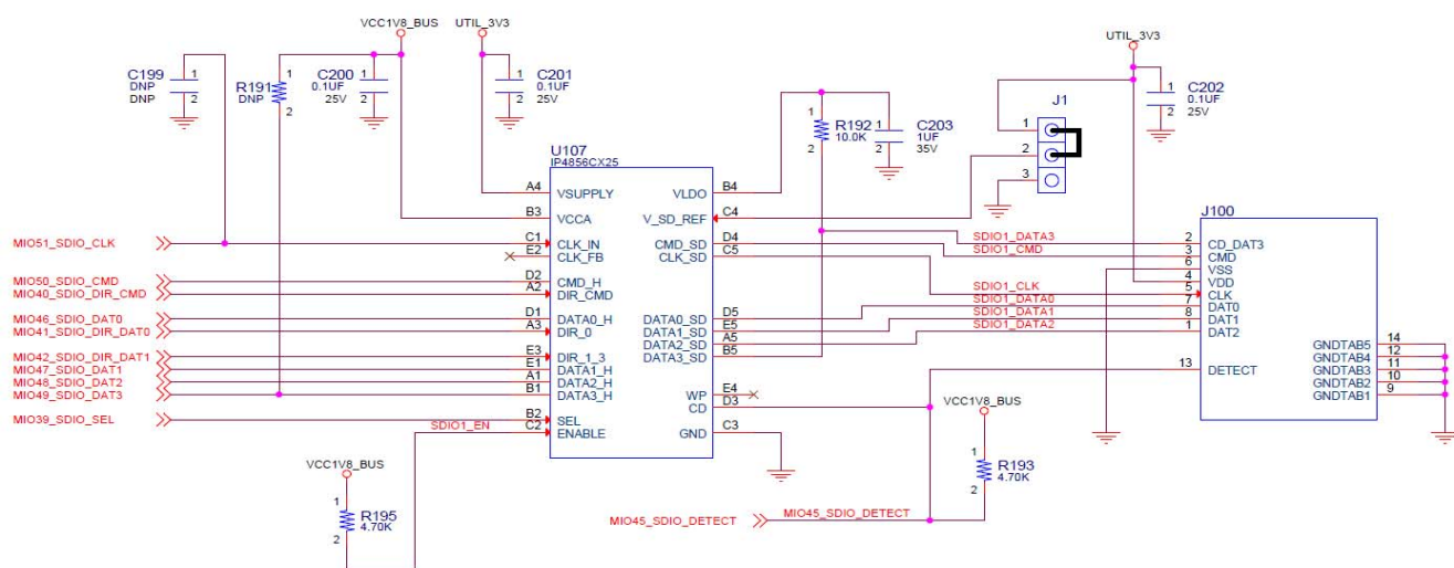
Figure 3-7: SD Card Interface
