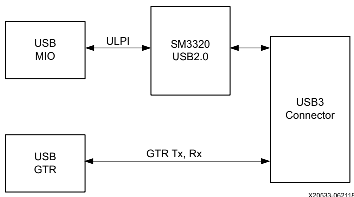
Figure 3-8: USB Interface
