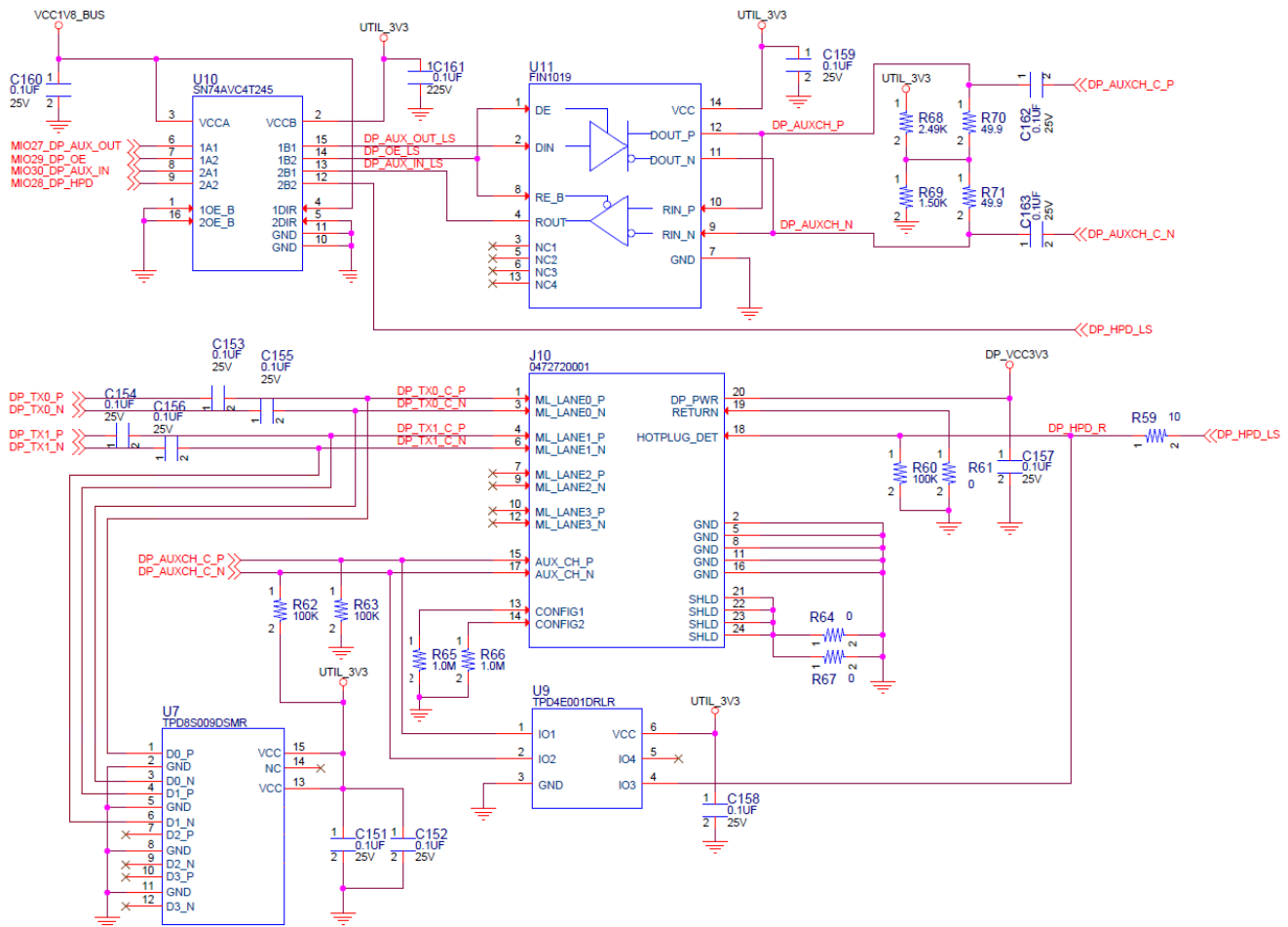
Figure 3-6: DisplayPort Circuit
