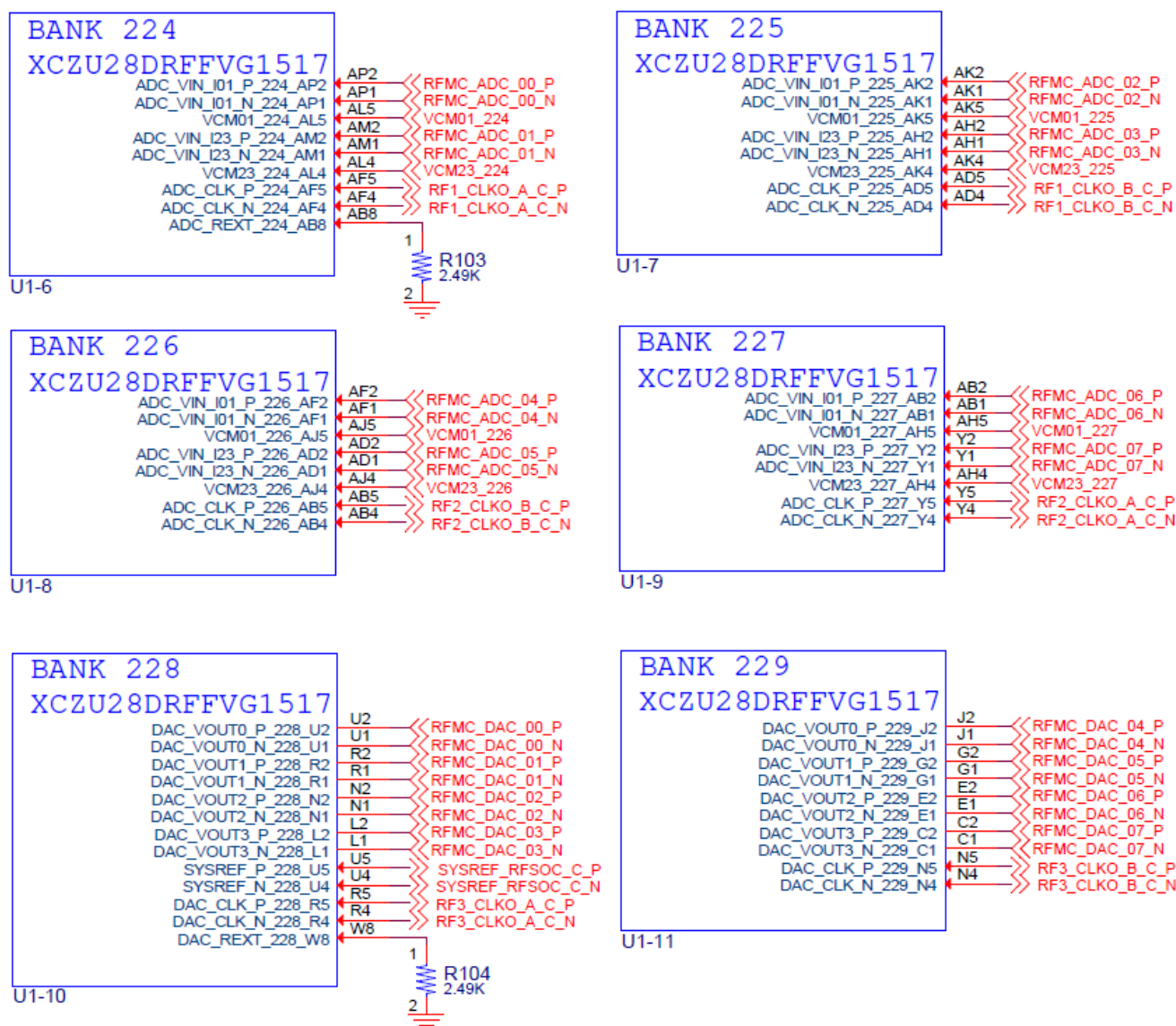
Figure D-4: RFSoc ZCU28DR ADC/DAC Banks 224-229 Connectivity
