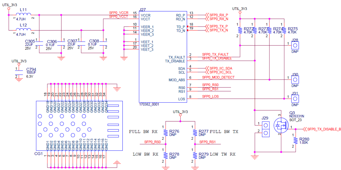
Figure 3-23: SFP28 Module Connectivity
