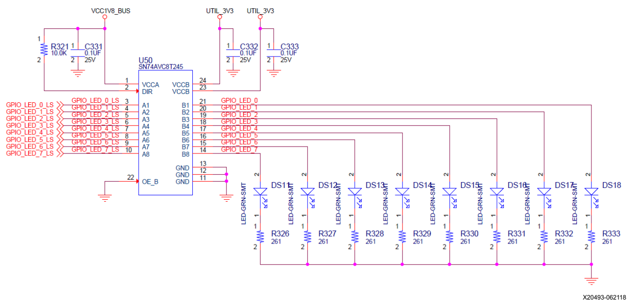
Figure 3-25: GPIO LEDs
