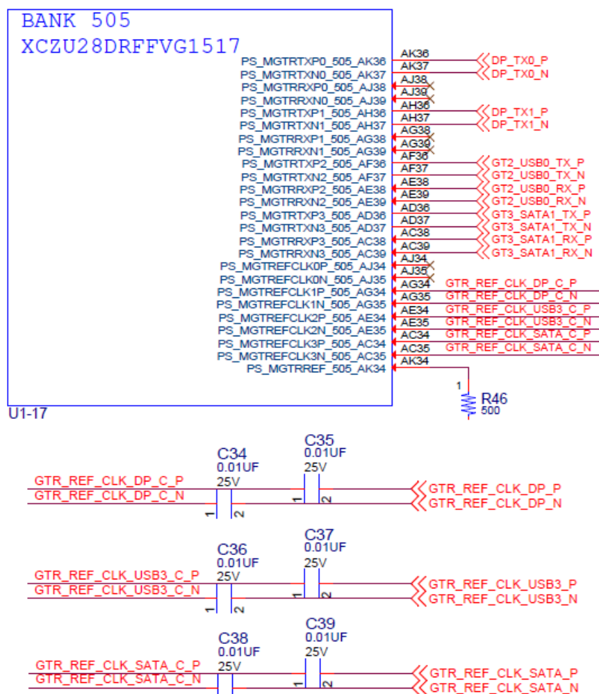
Figure 3-30: PS-GTR Lane Assignments
