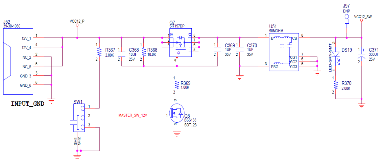
Figure 3-34: Power Input
