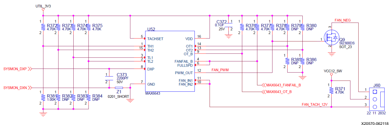
Figure 3-32: 12V Fan Header
