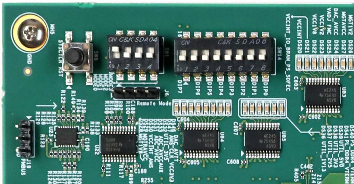
Figure 3-28: Power and Status LEDs
