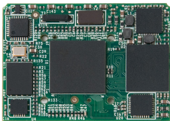
AM1808 SOM-M1
